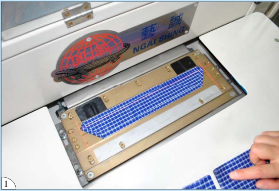
1. 下模抽風便於將裁片折邊、貼合完好 Vacuuming of the lower mould is suitable for fabric piece folding and jointing
